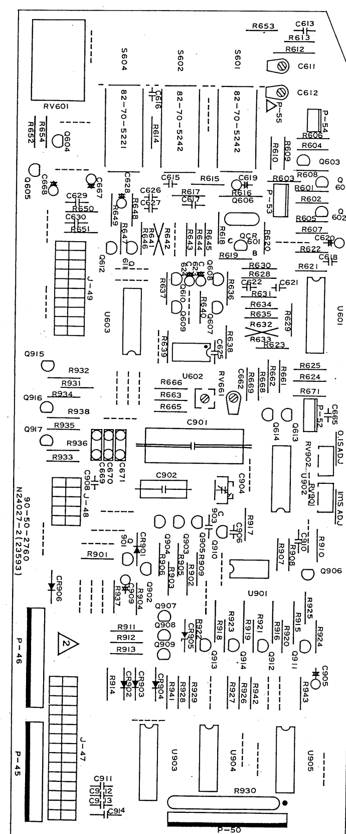
A8 B TRIG & B SWEEP Parts Location
