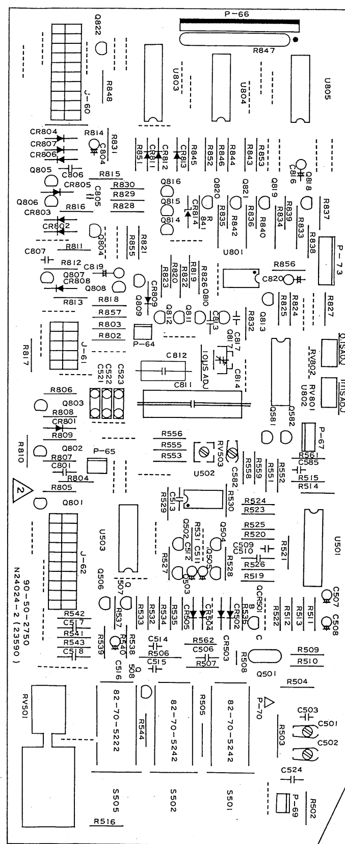
A7 A TRIG & A SWEEP Parts Location
