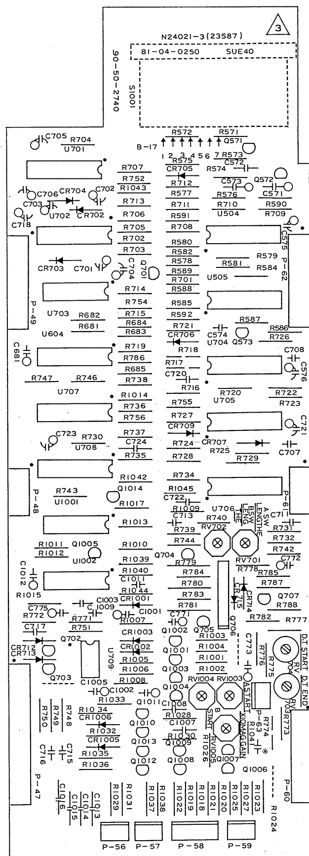
A6 TRIG & SWEEP CONTROL Parts Location
